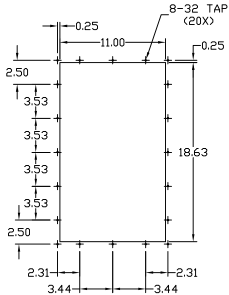
ENCLOSURE CUTOUT
