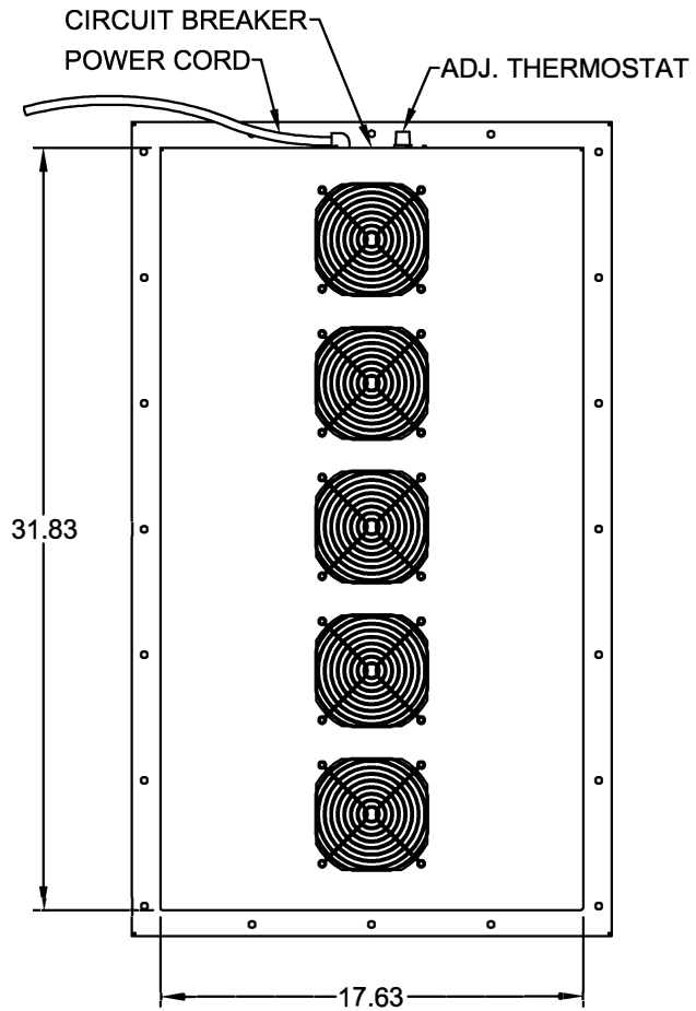
COLD SIDE VIEW (ENCLOSURE SIDE)
