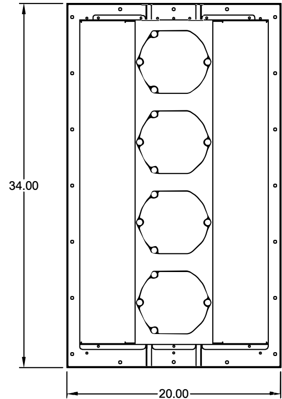
HOT SIDE VIEW (EXTERNAL SIDE)
