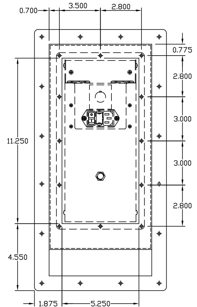
REAR VIEW
