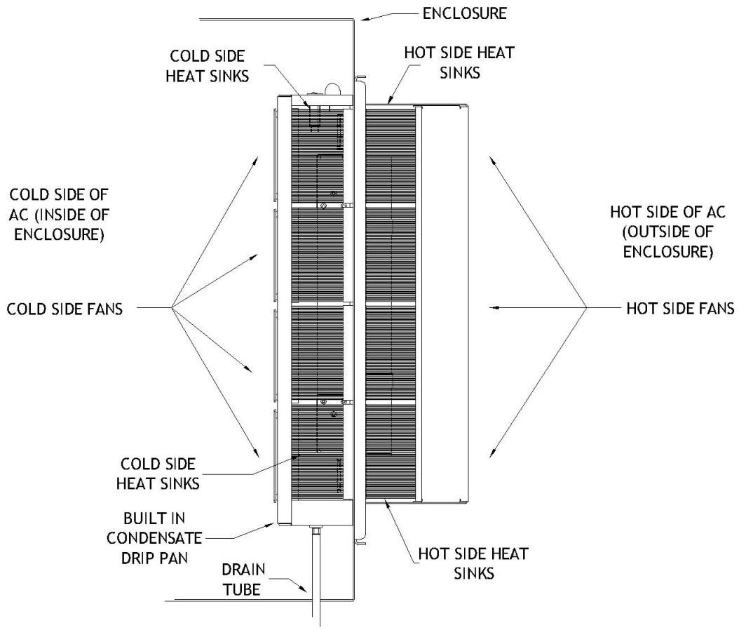
VERTICAL INSTALLATION OF 3500 BTU UNIT WITH INTEGRAL DRIP PAN AND DRAIN TUBE
