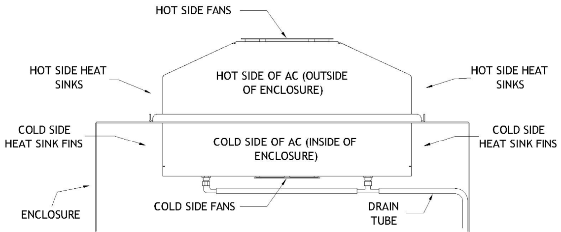
HORIZONTAL INSTALLATION OF 3500 BTU UNIT WITH INTERNALLY MOUNTED DP-161H DRIP PAN AND DRAIN TUBE
