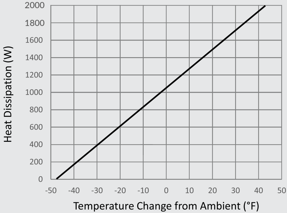
AAC-161B Performance Chart
