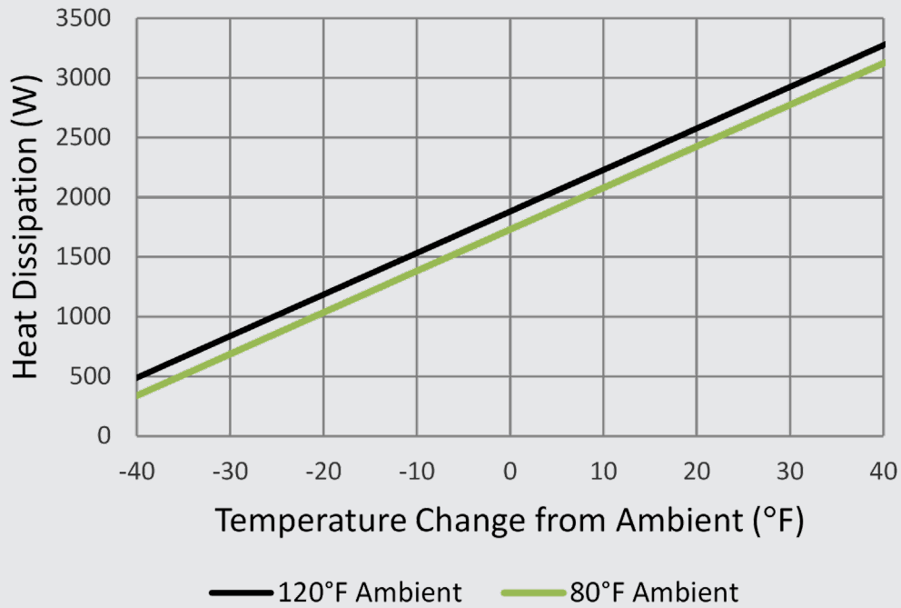
AAC-170 Performance Chart
