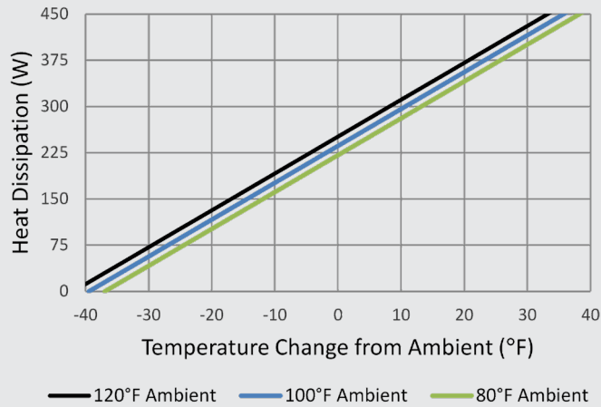
AAC-141A Performance Chart
