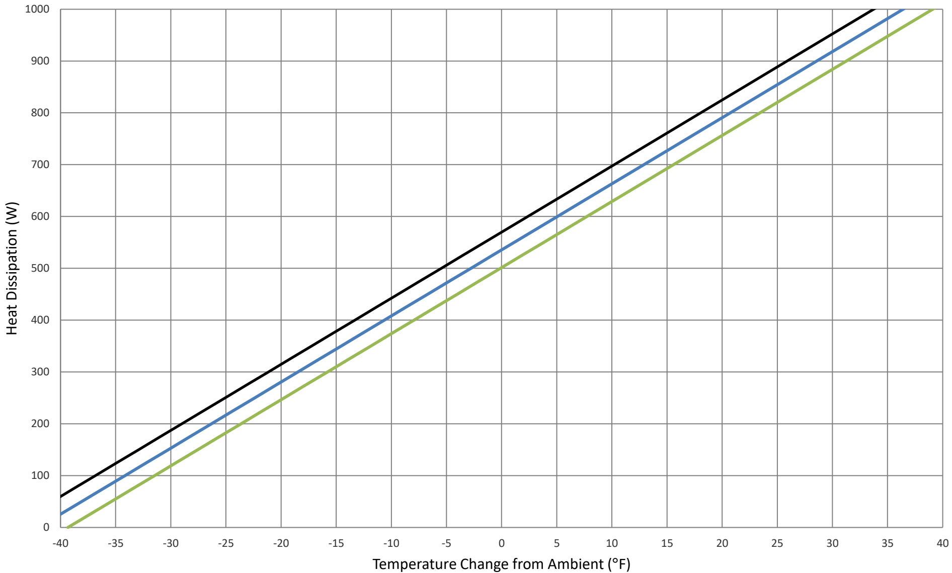
AAC-145A Performance Chart
