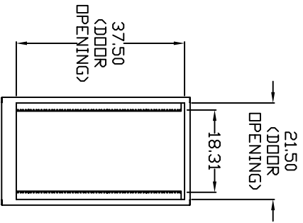
FRONT VIEW WITH DOOR REMOVED
