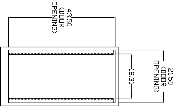
FRONT VIEW WITH DOOR REMOVED
