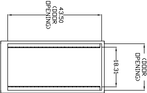
FRONT VIEW WITH DOOR REMOVED
