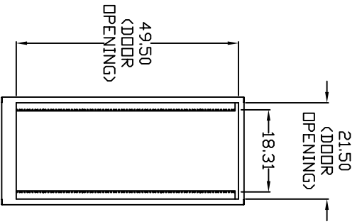
FRONT VIEW WITH DOOR REMOVED
