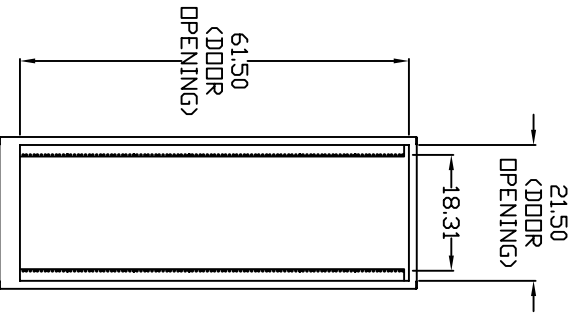
FRONT VIEW WITH DOOR REMOVED
