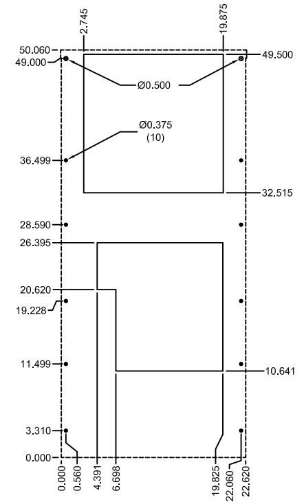
CUTOUT DRAWING
