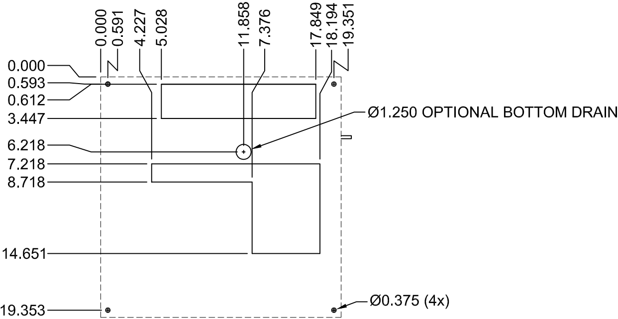
CUTOUT DRAWING
