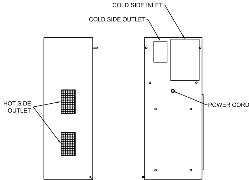
REAR VIEW
