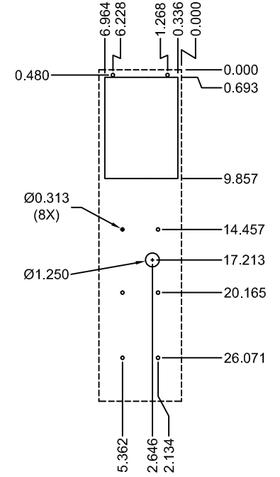
CUTOUT DRAWING
