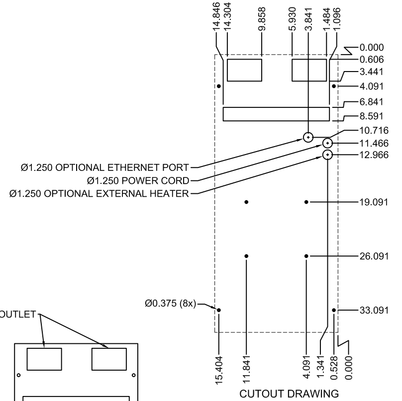
CUTOUT DRAWING
