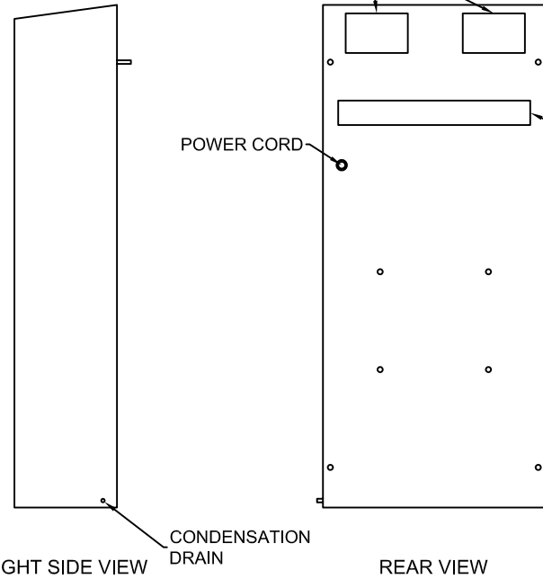
REAR VIEW
