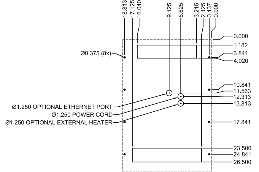
CUTOUT DRAWING
