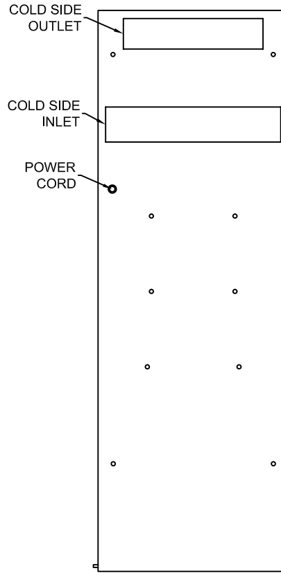
REAR VIEW
