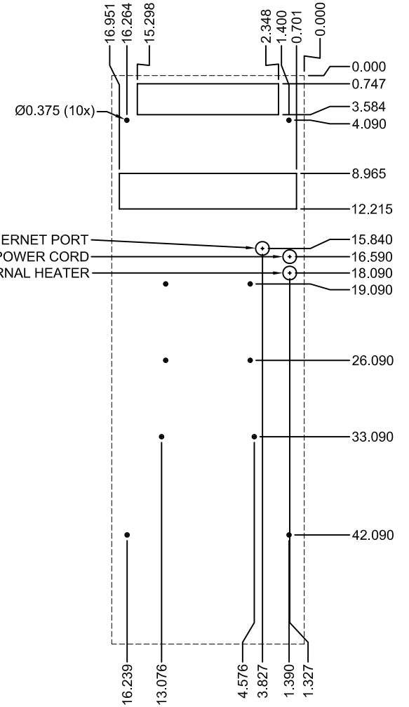
CUTOUT DRAWING
