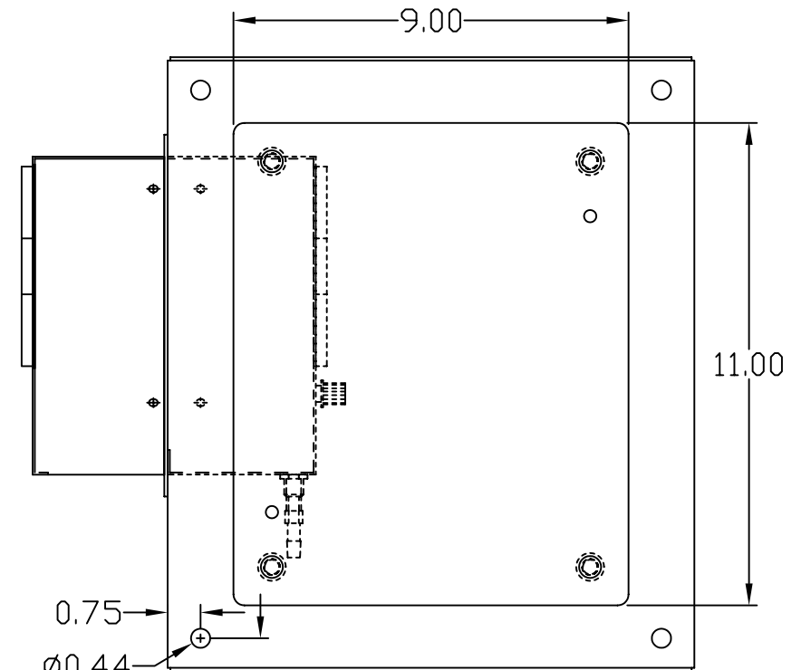
REAR VIEW
