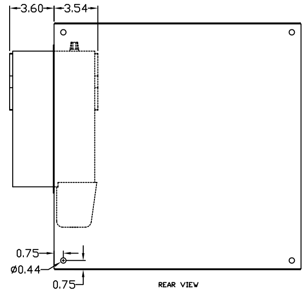
REAR VIEW
