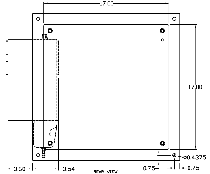
REAR VIEW
