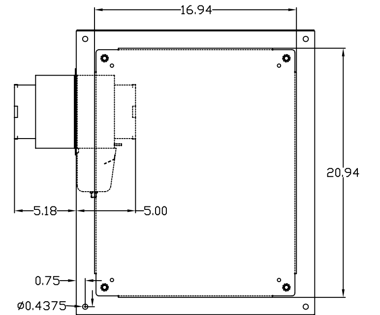
REAR VIEW
