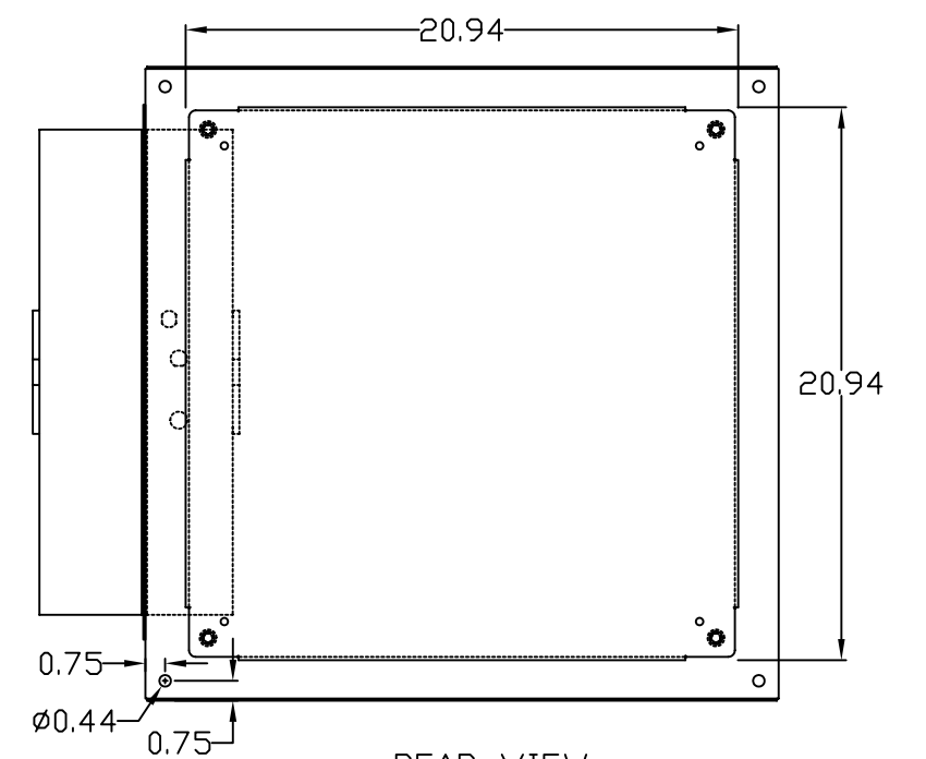
REAR VIEW
