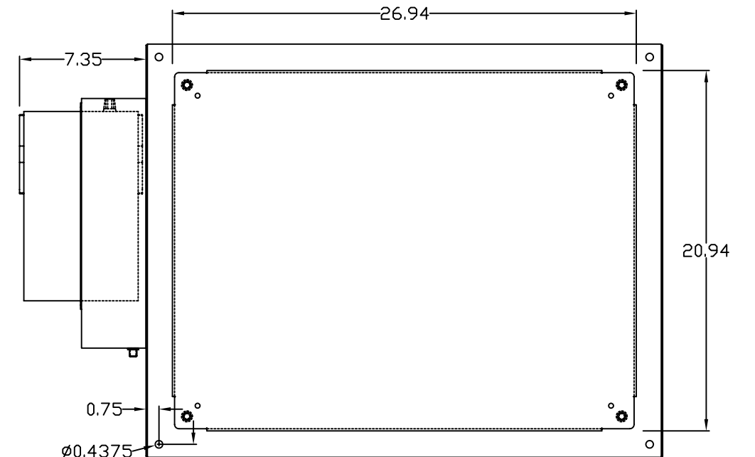
REAR VIEW
