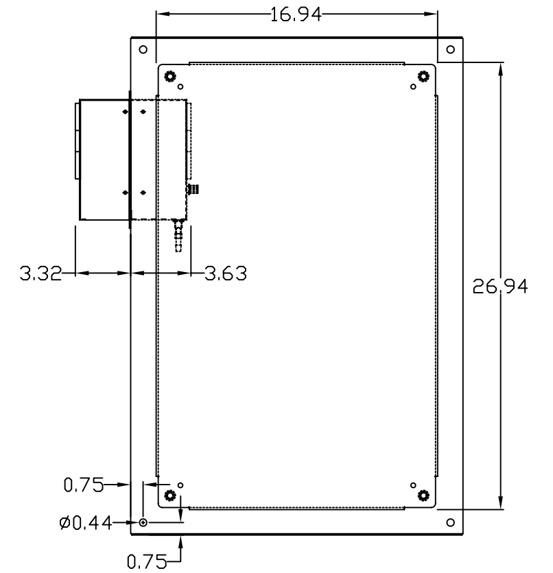
REAR VIEW
