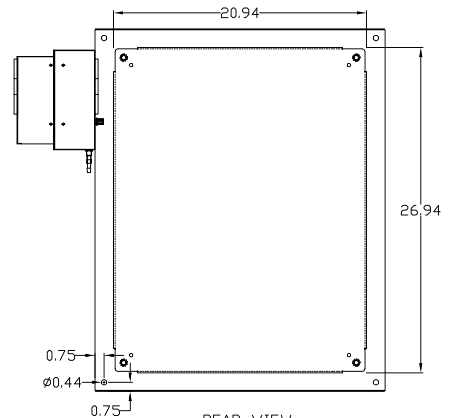
REAR VIEW
