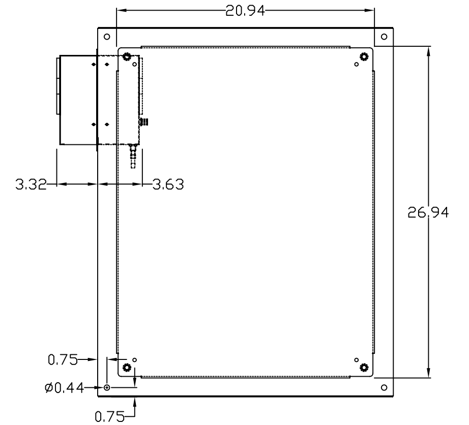
REAR VIEW
