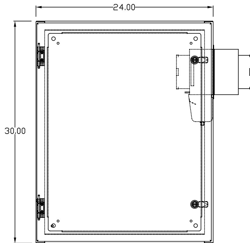
FRONT VIEW
