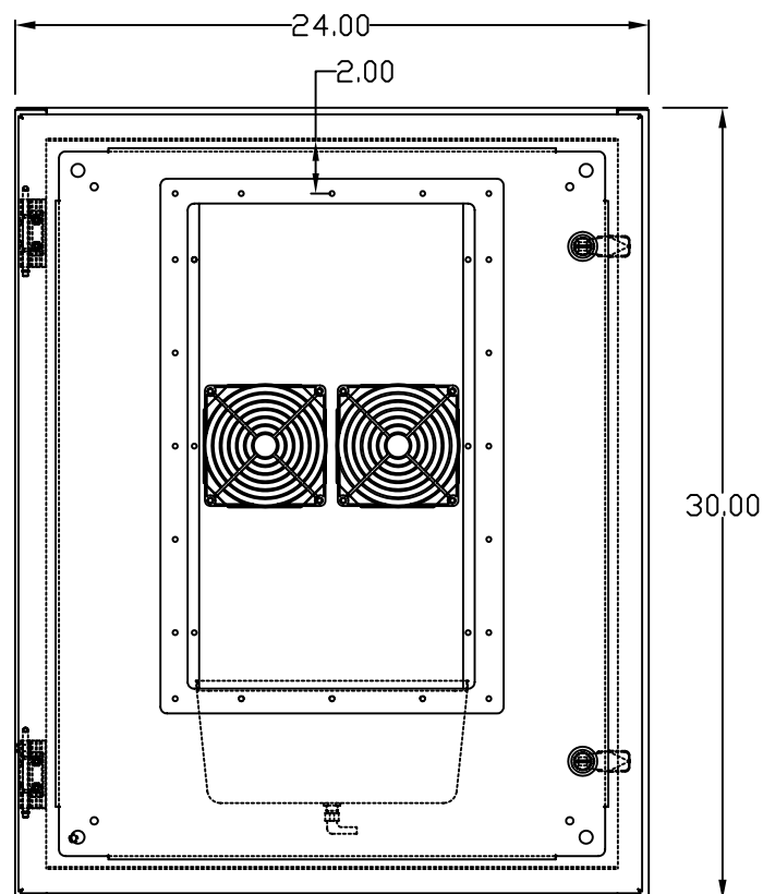
FRONT VIEW
