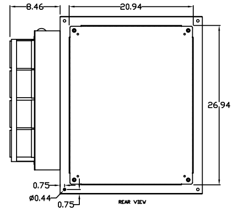
REAR VIEW
