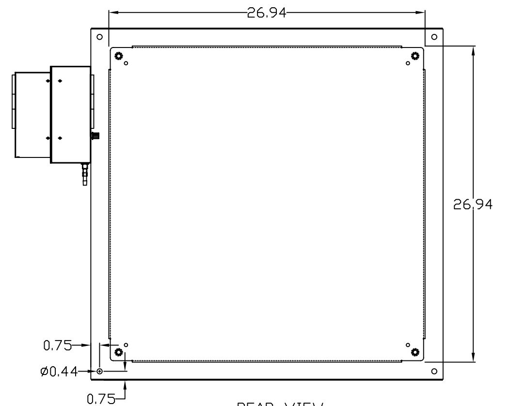
REAR VIEW
