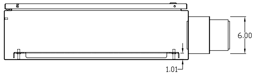
BOTTOM VIEW
