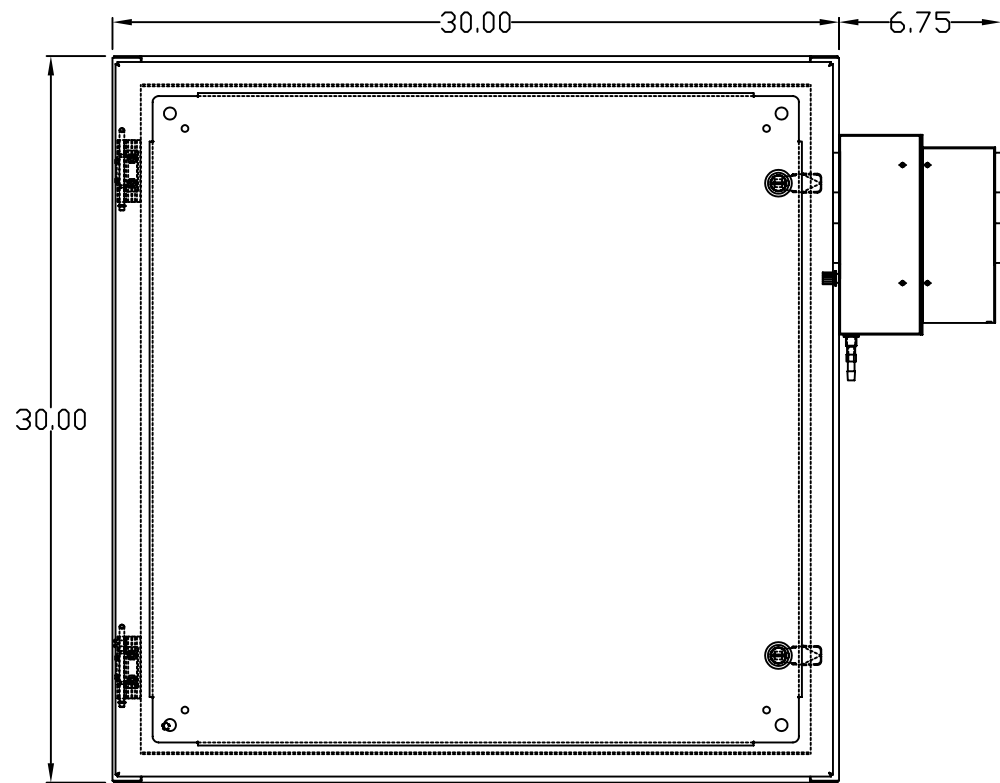
FRONT VIEW
