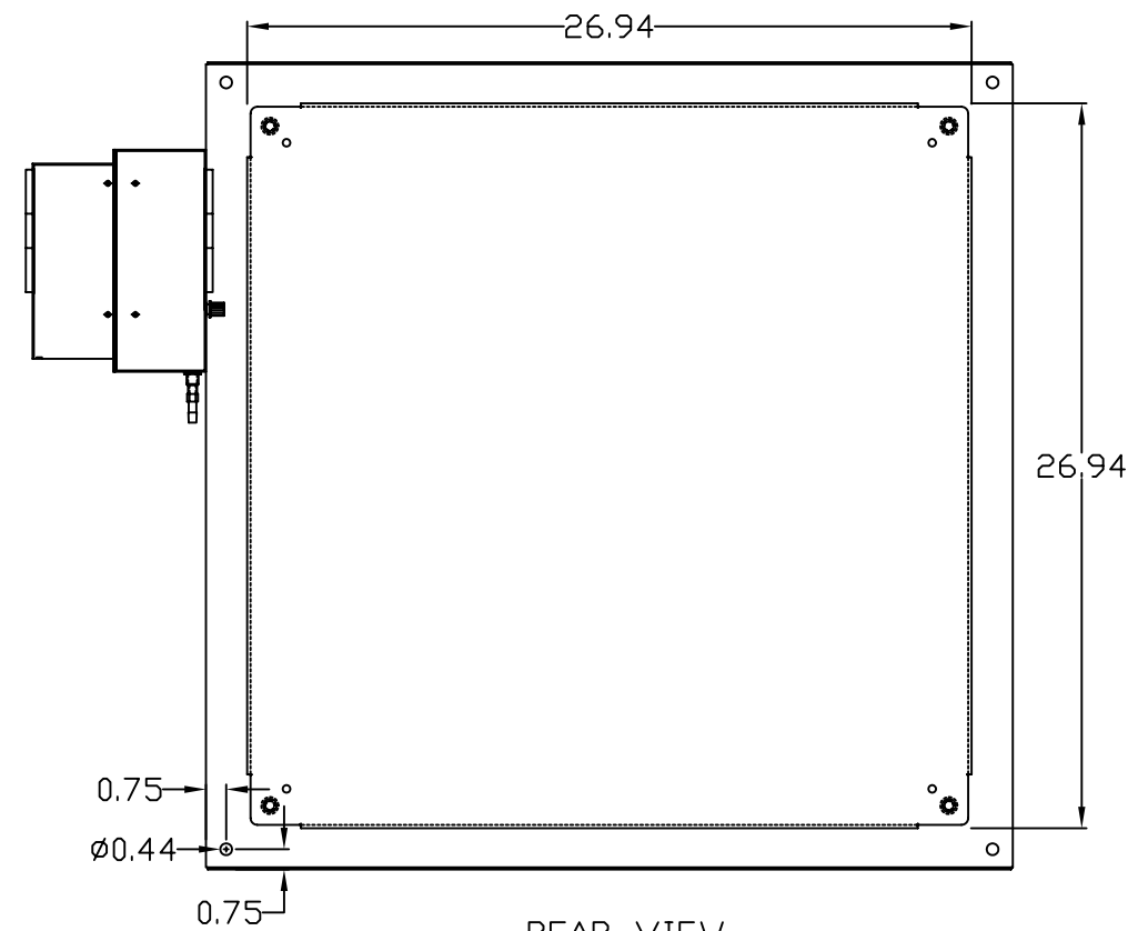
REAR VIEW
