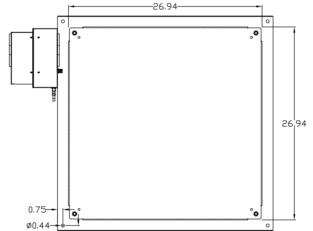
REAR VIEW
