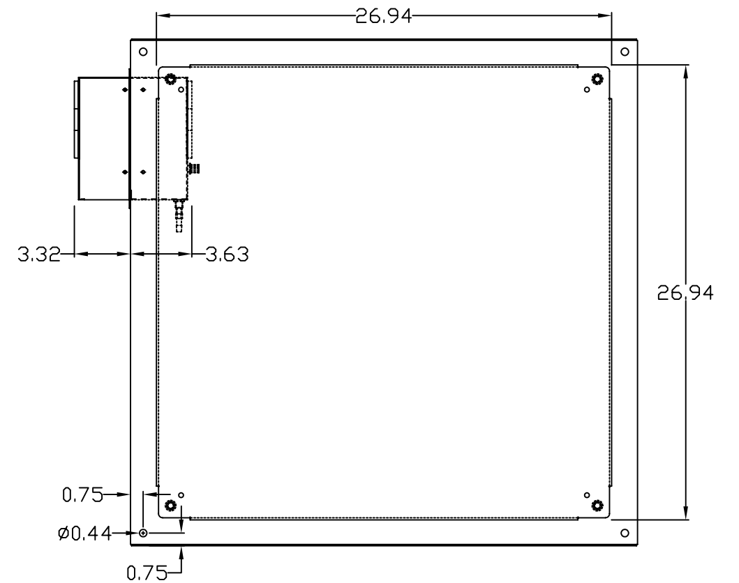
REAR VIEW
