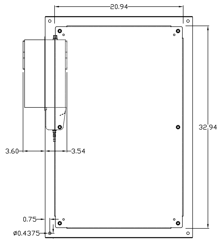
REAR VIEW
