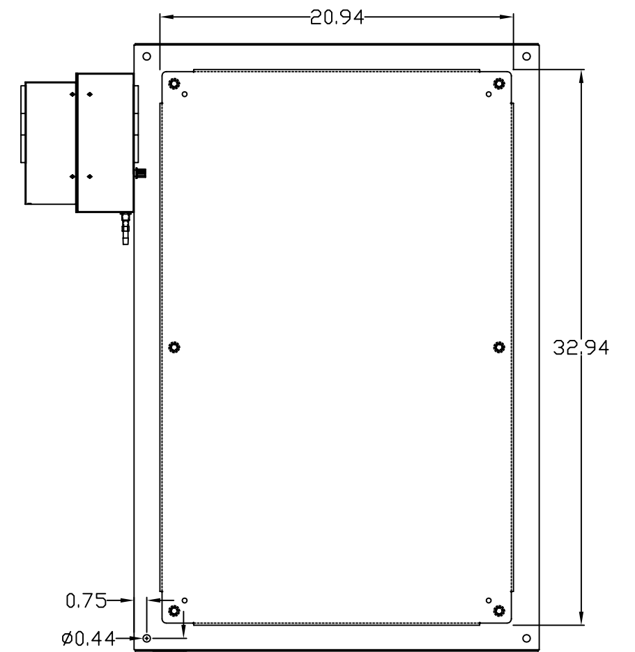
REAR VIEW
