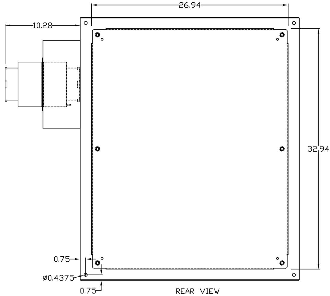
REAR VIEW
