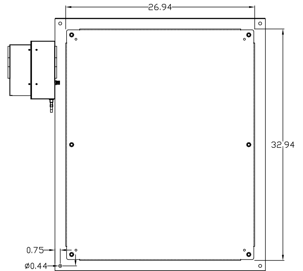
REAR VIEW
