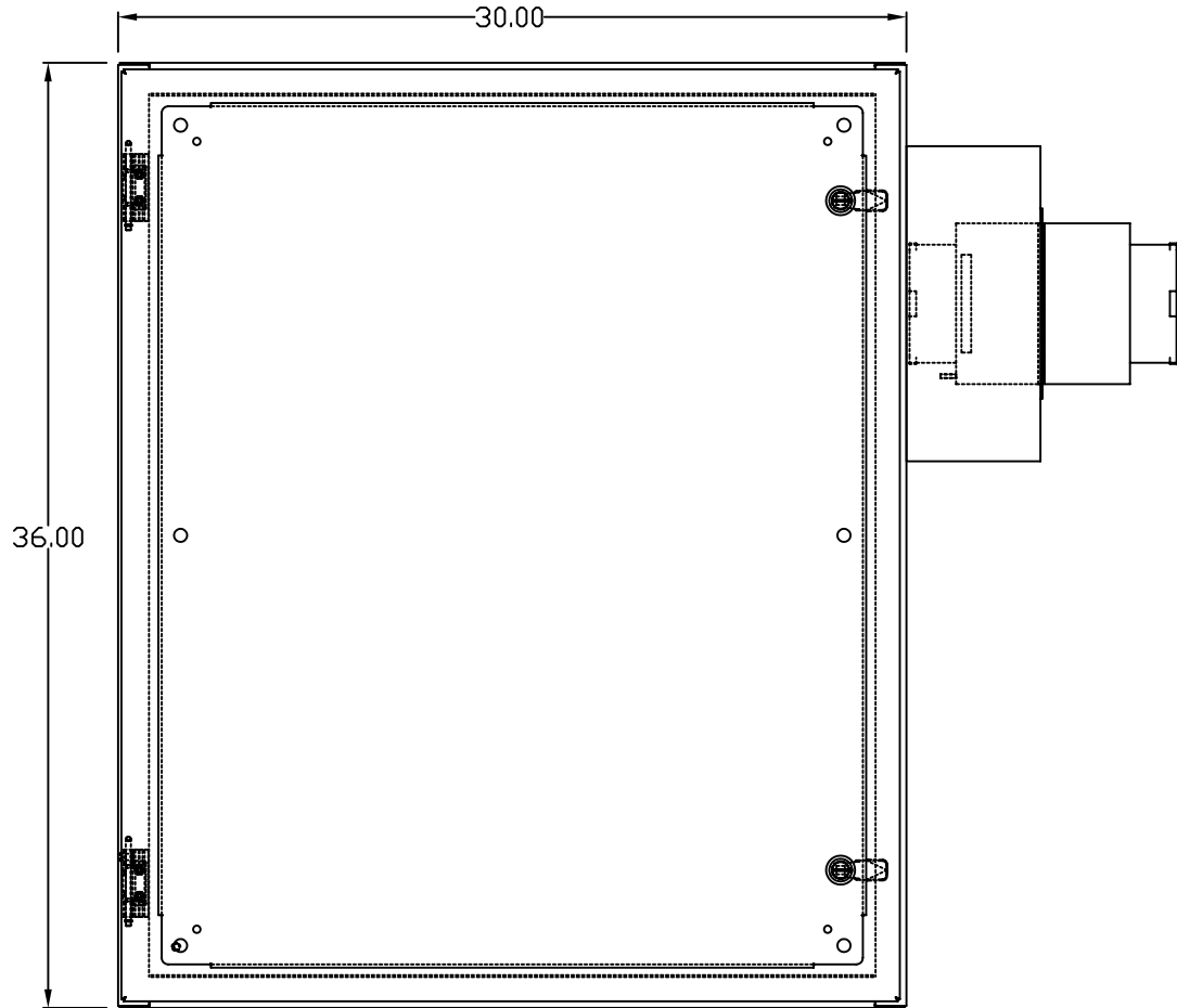
FRONT VIEW
