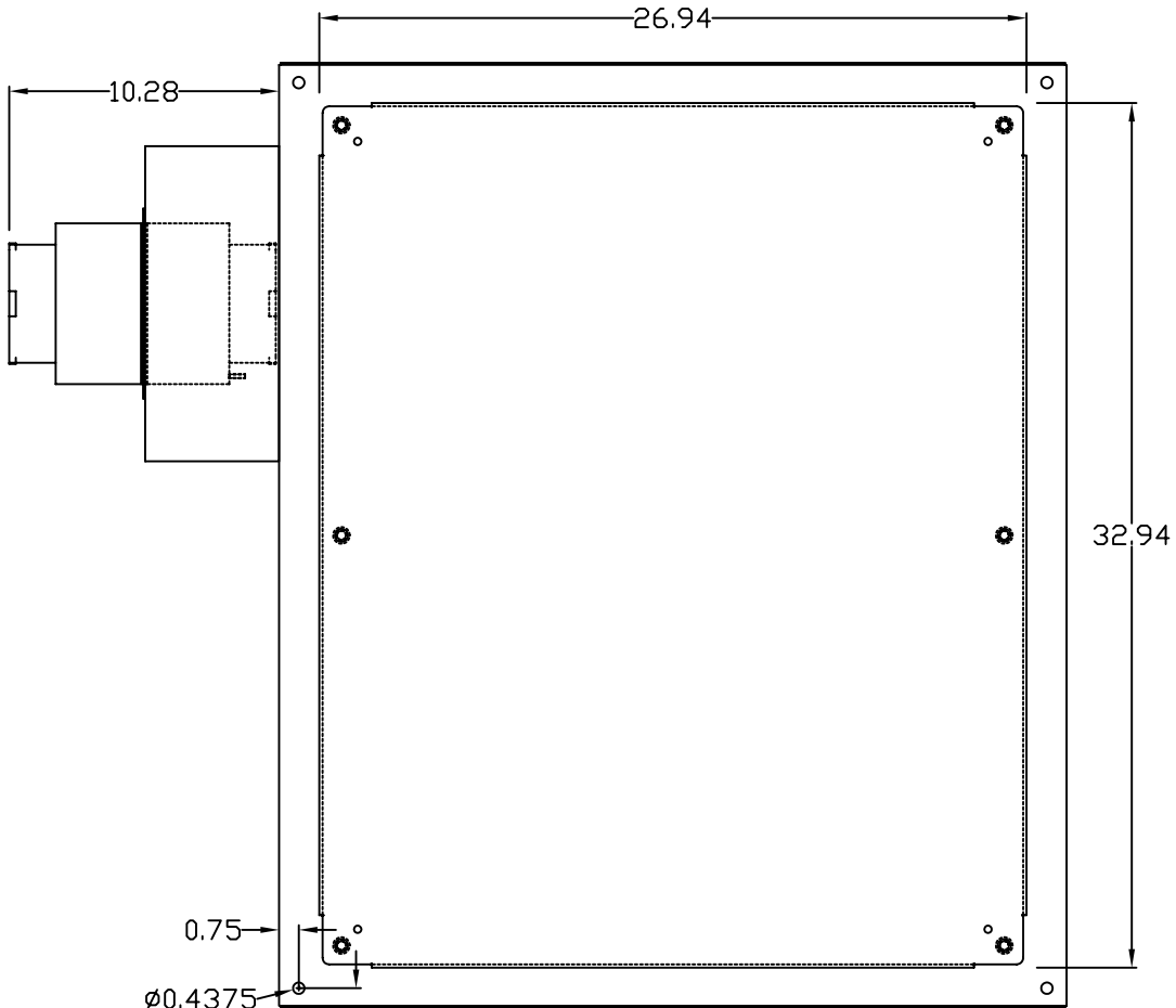
REAR VIEW
