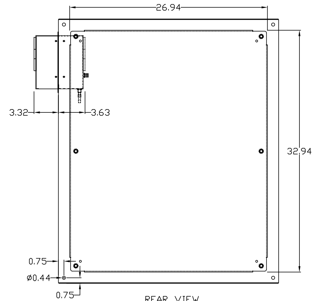
REAR VIEW
