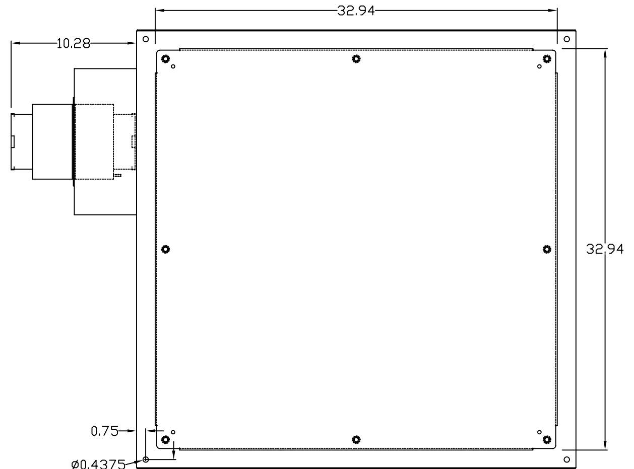
REAR VIEW
