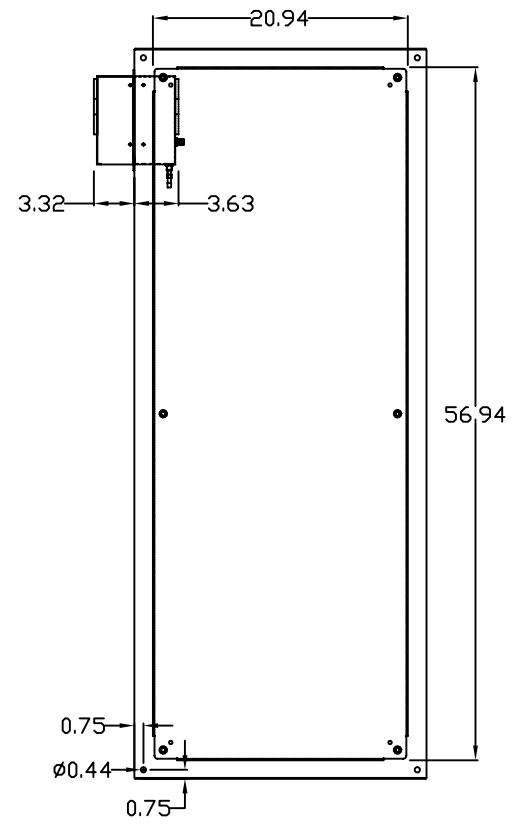
REAR VIEW
