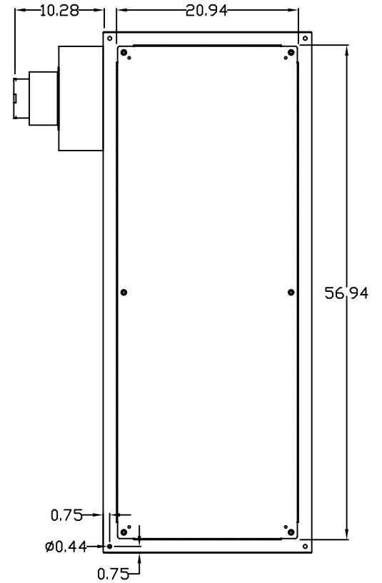
REAR VIEW
