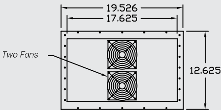
Hot Side (External to Transit Case)
