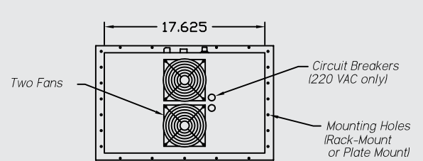
Cold Side (Internal to Transit Case)
