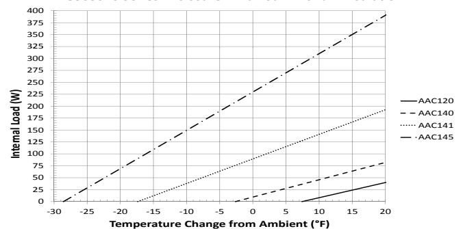
1G363016 Series Enclosure in Full Sun with ¾" Insulation
