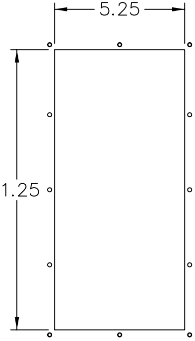
Cabinet Cutout
