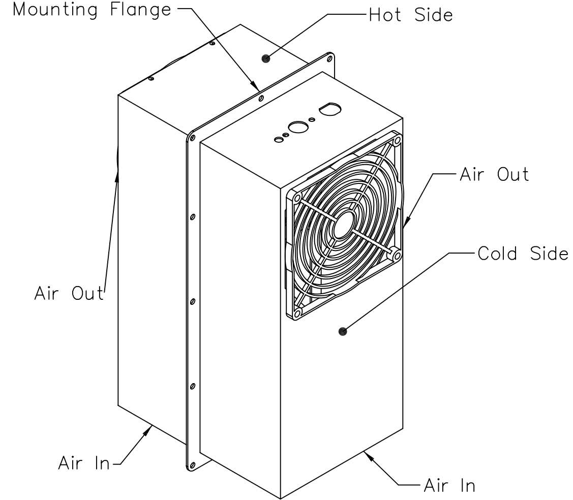
Preferred Orientation
